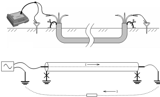
Fig.3.1 Conductor-Earth Connection Method
