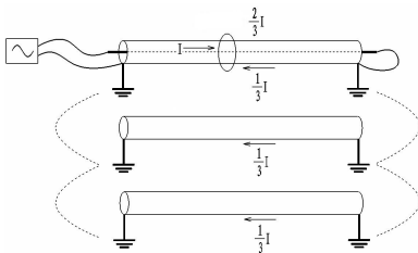
Fig.3.4 External effect: 2/3 I
